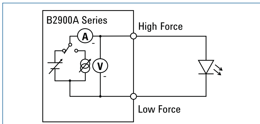
Figure 1. Using the B2900A Series to characterize an LED
